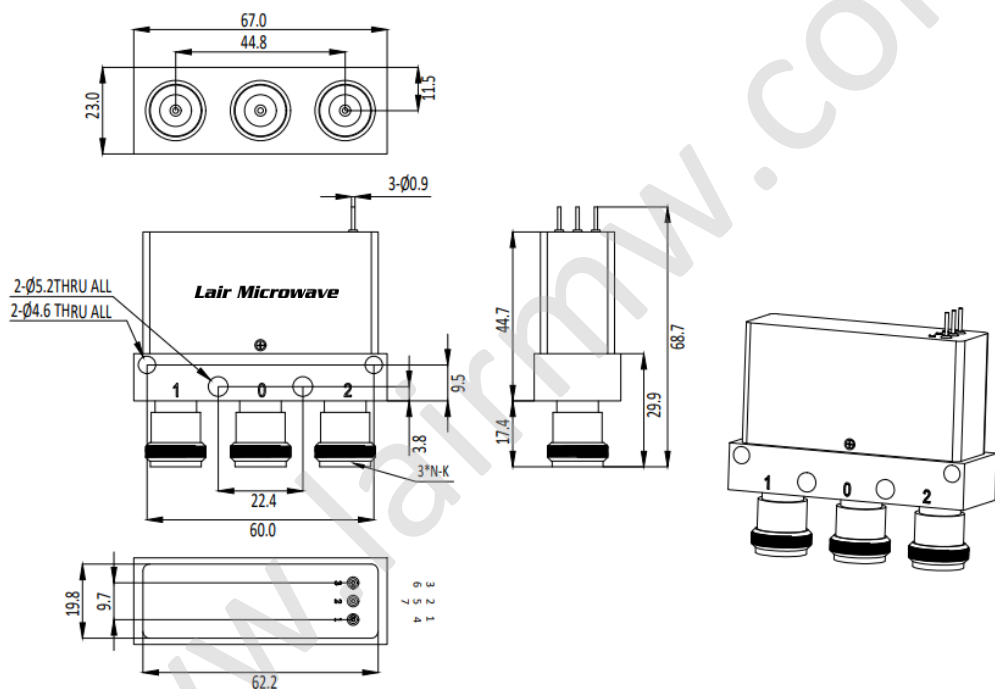
引脚编号 PIN No. 定义 Definition TTL 输入 TTL Input 射频通道 RF Continuity "1" +12V - RF 0↔1 "2" GND - "3" TTL High Level RF 0↔2 初始状态下, RF0↔1 常闭 In the initial state, RF 0↔1 is normally closed.
