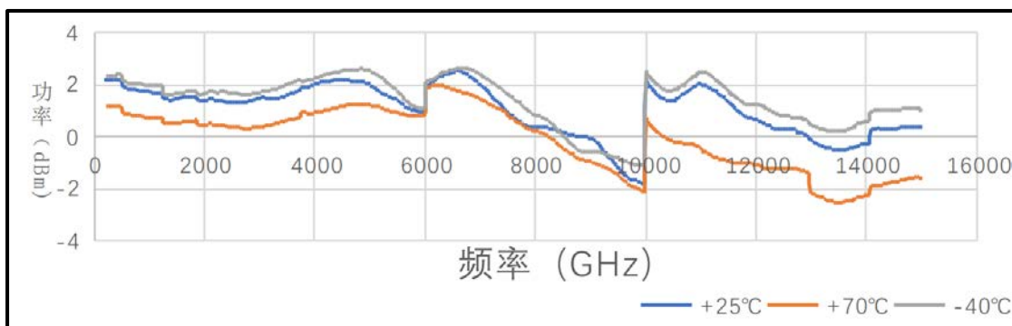
LFS-1003 输出功率 Output Power
