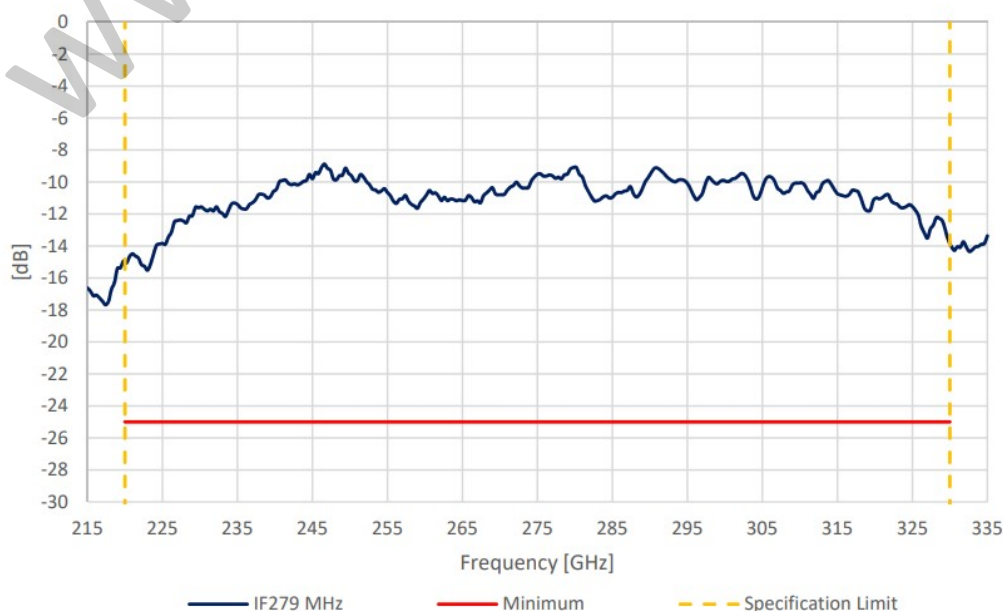
Conversion Loss(SSB) vs Frequency
